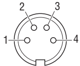
M16 Female 4p molded connector Front View
